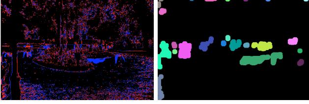
Figure 3. Motion map generated from Fig. 1(a). Left image shows M^* ; please note that non-black pixels are the ones marked for motion detection refinement. Right image shows M after the application of the morphological operations; each cluster is coded with a different index, which in the figure is represented by a colour.
